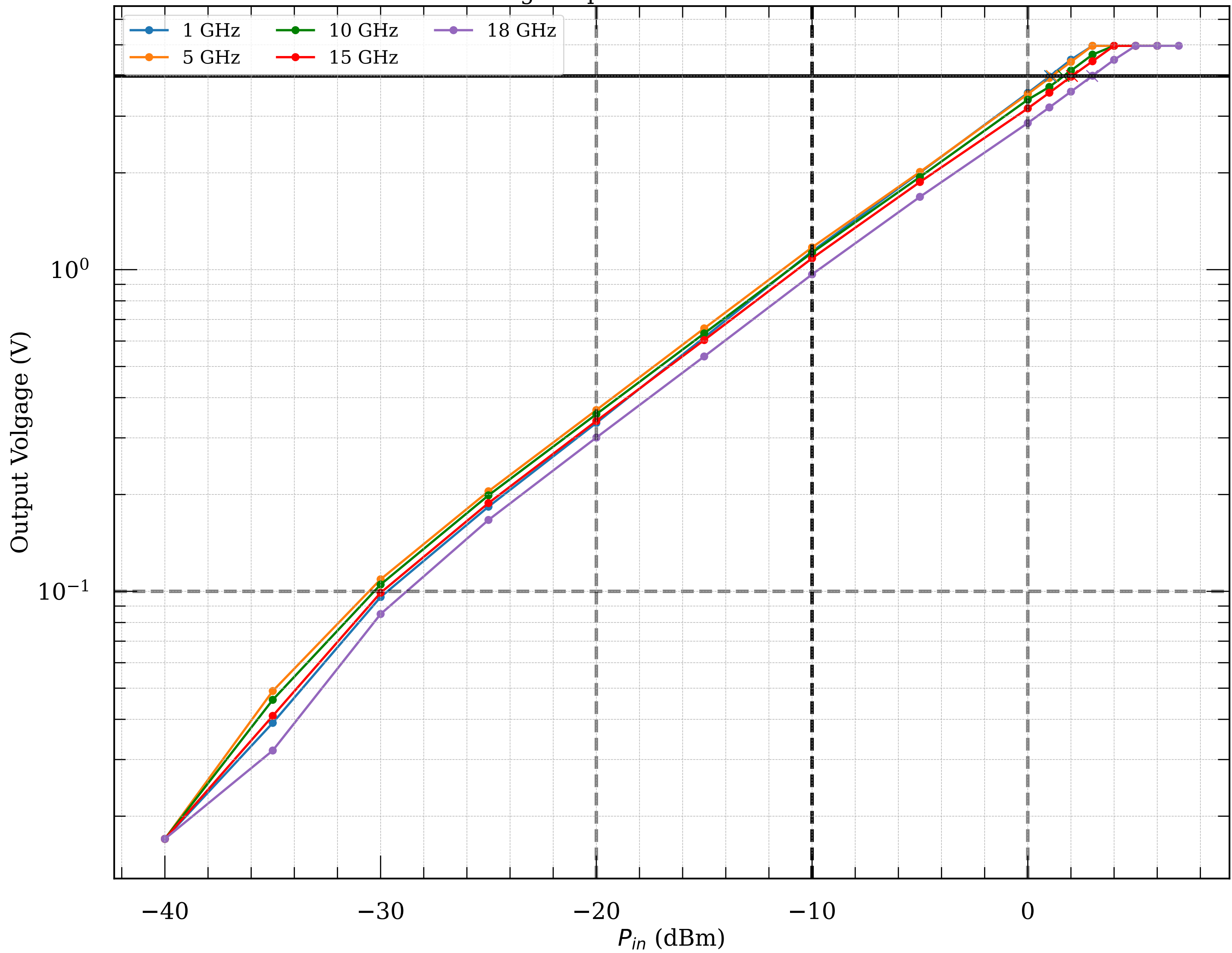
Measured voltage-to-power curve of detector module029
